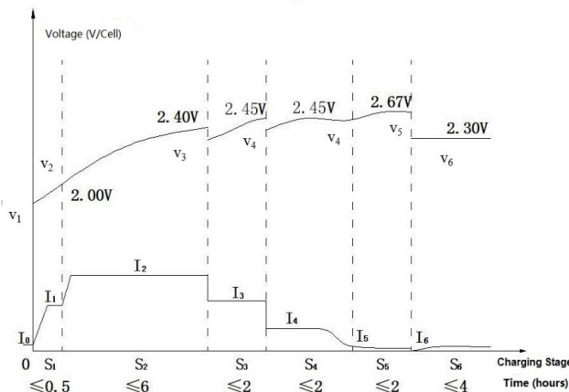
Charge Curve for 6-EVF-70T (for Single Cell)
